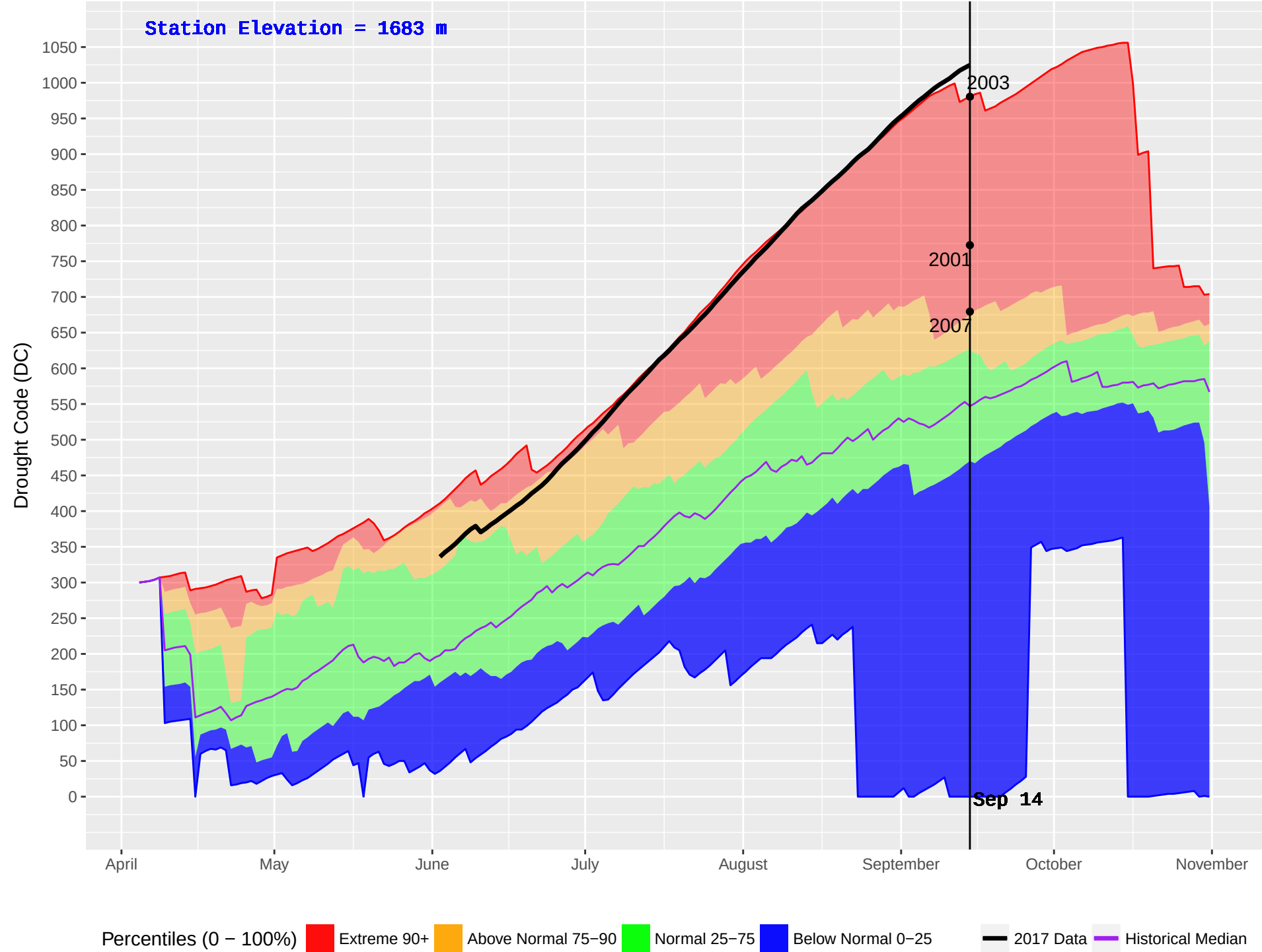
ASHNOLA (331) : Historical (1992–2016) and Current (2017) Noon Drought Code (DC)
